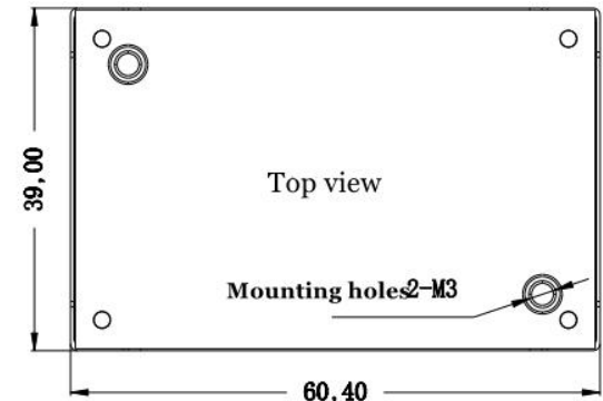
Standard 60.4*39*12.7mm
