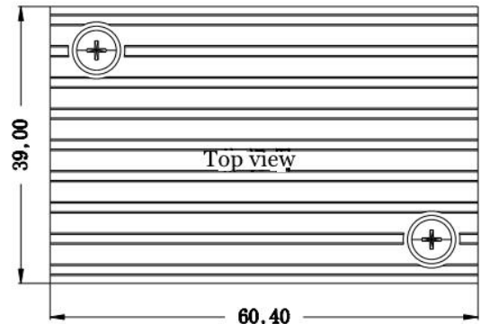
Standard+Heatsink 60.4*39*27.7mm
